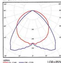
Luminaire: MWP3T5_6_28CS -AL01 Lamps: 3 x Fluor. 28W 4' Silhouette T5
