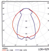
Luminaire: MWP2_T5_6_28CS_AL01_MB Lamps: 2 x Fluor. 28W 4' Silhouette T5
