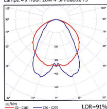
Luminaire: MWP4T5_6_28CS -AL01 Lamps: 4 x Fluor. 28W 4' Silhouette T5
