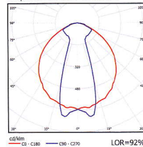
Luminaire: MWP2_T5_6_28CS_AL01 Lamps: 2 x Fluor. 28W 4' Silhouette T5
