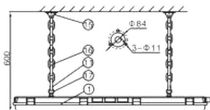
Chain type
