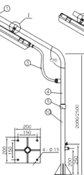
Flange type
