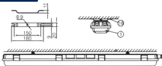
Ceiling type
