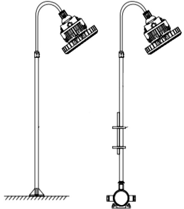
Stanchion Type
